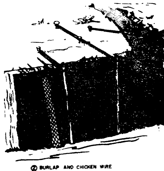
Figure 2-21. Types of metal revetment.
